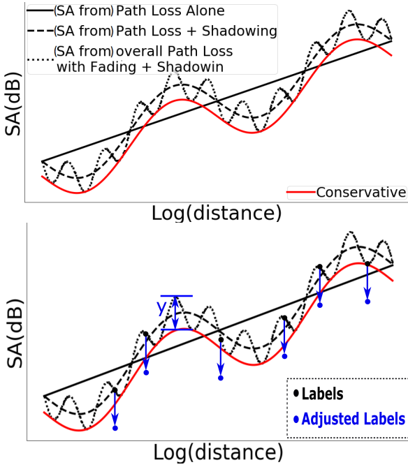
FIGURE 5: (a) Spectrum allocation function, when there is a single PU and a single SU, due to path loss with shadowing and multi-path fading effects. Note that the path-loss function has a similar trend. The red plot is a conservative spectrum allocation, based on a similar conservative path-loss function. (b) Modifying labels of training samples to drive the model towards learning a simpler and more conservative spectrum allocation function.
