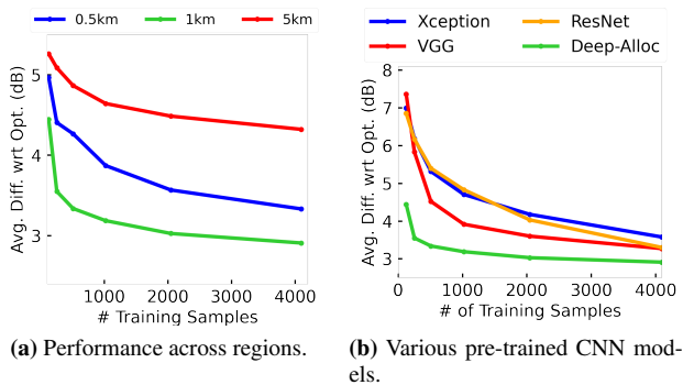
FIGURE 10: Performance comparison of (a) DeepAlloc over different regions, and (b) various pre-trained models for increasing number of training samples.
