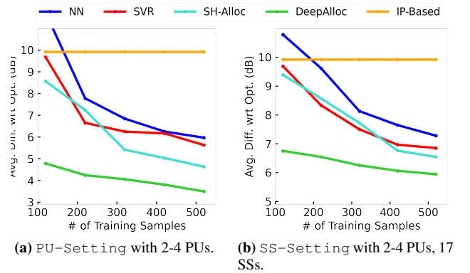
FIGURE 15: Testbed performance for increasing training set.
