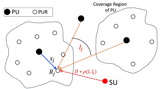
FIGURE 1: Eqn. (1) Illustration. The optimal power that can be allocated to an SU is such that, at each PUR (a PU's receiver) the signal-to-noise ratio is more than the desired ratio, \beta . Above, R_j is a certain PUR, I_j is the total interference at R_j from other PUs, s_j is the signal strength received at R_j from its PU, and \Pi \cdot \rho(l, l_j) is the interference due to the SU at R_j where l and l_j are their respective locations.
