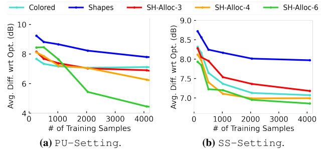
FIGURE 7: Performance comparison of various schemes for pre-processing the training samples into images.
