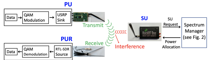
FIGURE 14: Testbed system overview, including the GNU-Radio based PU-to-PUR communication system.
