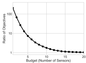
Fig. 9. Values of k (from Lemma 3) for varying budget.
